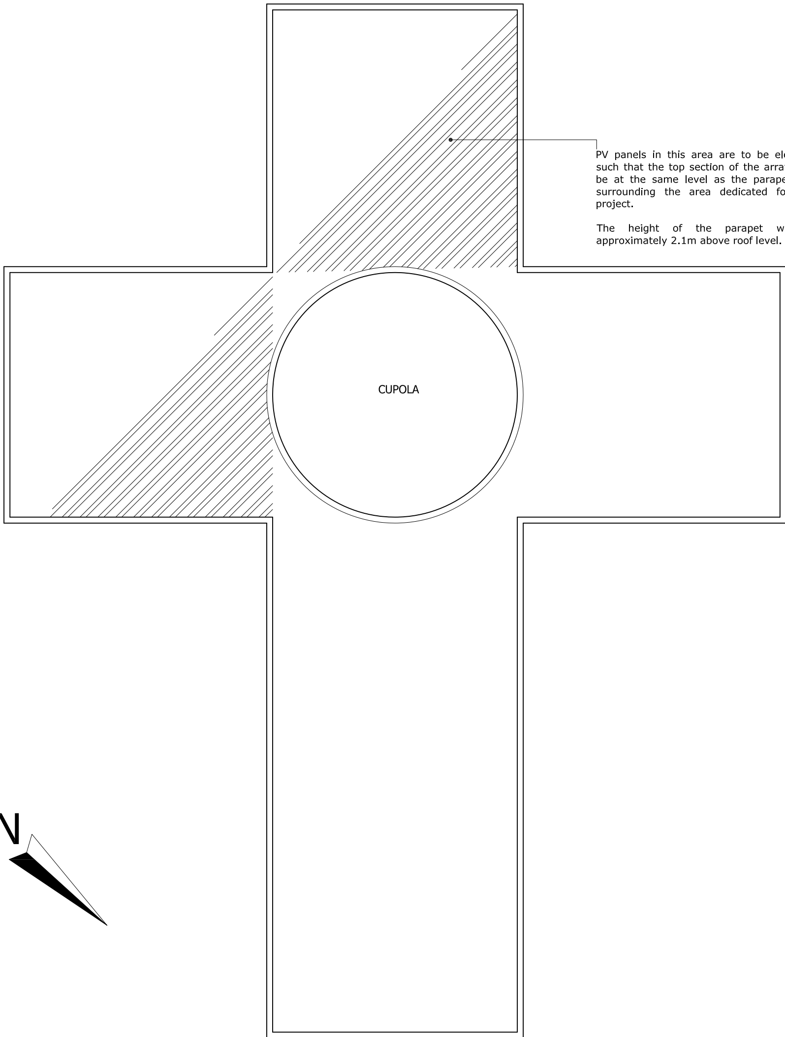
Roof Plan - Ghajnsielem Parish Church Scale 1:100
